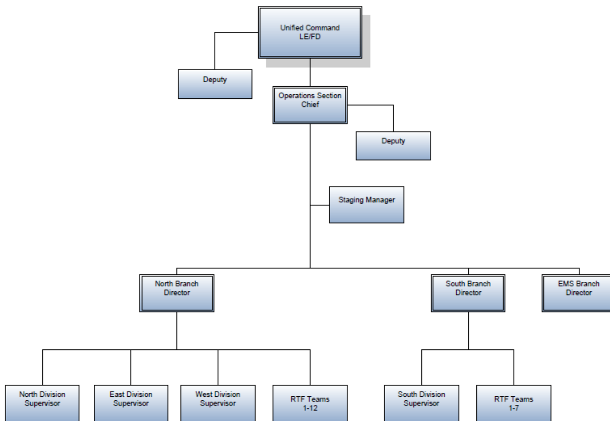
Figure 12: CCFD Unified Command Structure for 1 October
